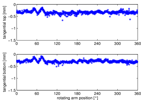
Fig. 27: slant, tangential deviations, 120°/s (cw)
