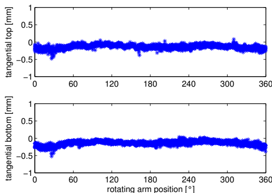
Fig. 19: horizontal, tangential deviations, 20°/s (cc)
