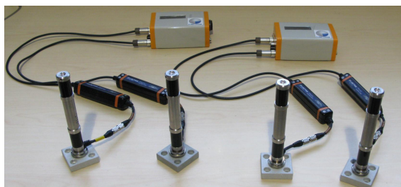
Fig. 5: Mini-vector bar, amplifier and PCE
